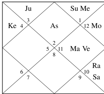
Ghatika Lagna 03:07:20
