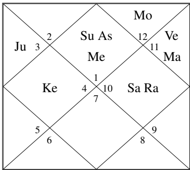
Bhava Lagna 13:43:33
